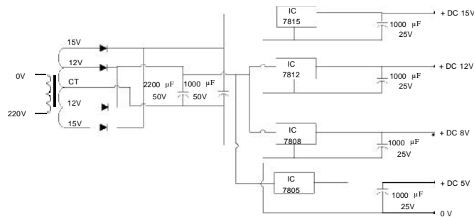
Gambar 6. Rangkain Catu Daya ( Power Supply )
